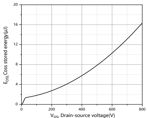
Figure 12. Typ. Coss stored energy
