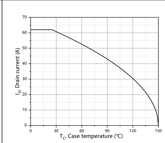
Figure 10. Drain current
